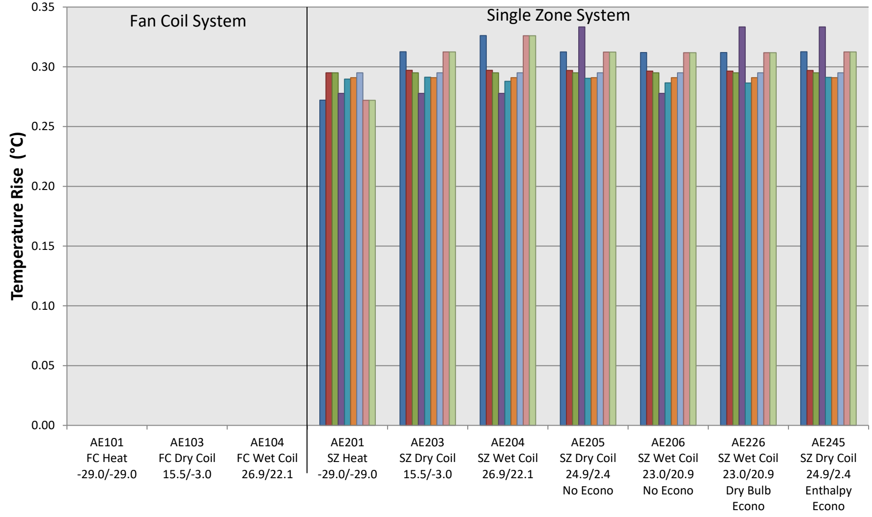
Figure B16.7.1-20. FC/SZ Return Fan Air Temperature Rise
