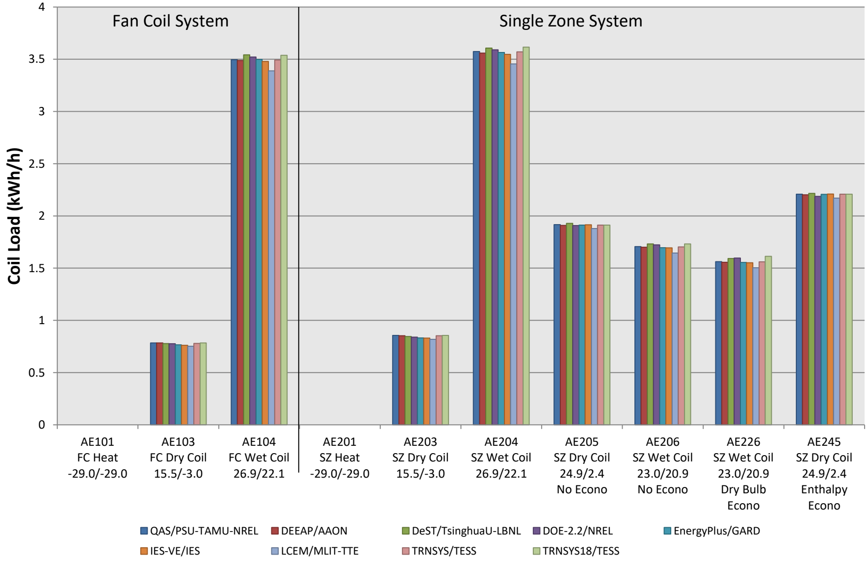
Figure B16.7.1-3. FC/SZ Cooling Coil Load, Sensible [QC_sensible]
