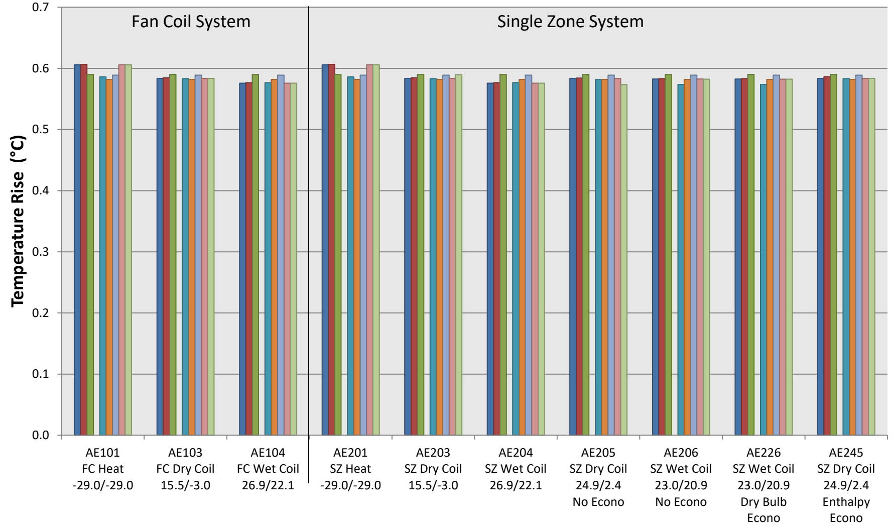
Figure B16.7.1-10. FC/SZ Supply Fan Air Temperature Rise
