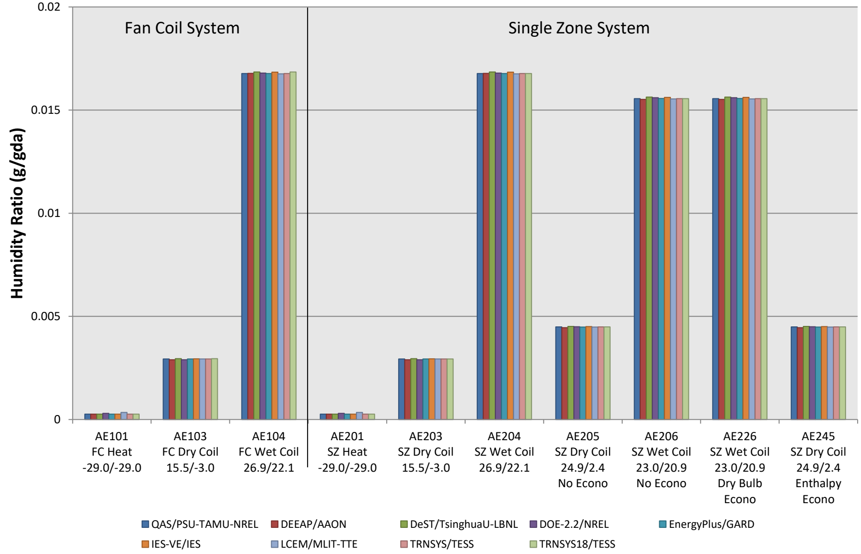
Figure B16.7.1-6. FC/SZ Outdoor Air Humidity Ratio
