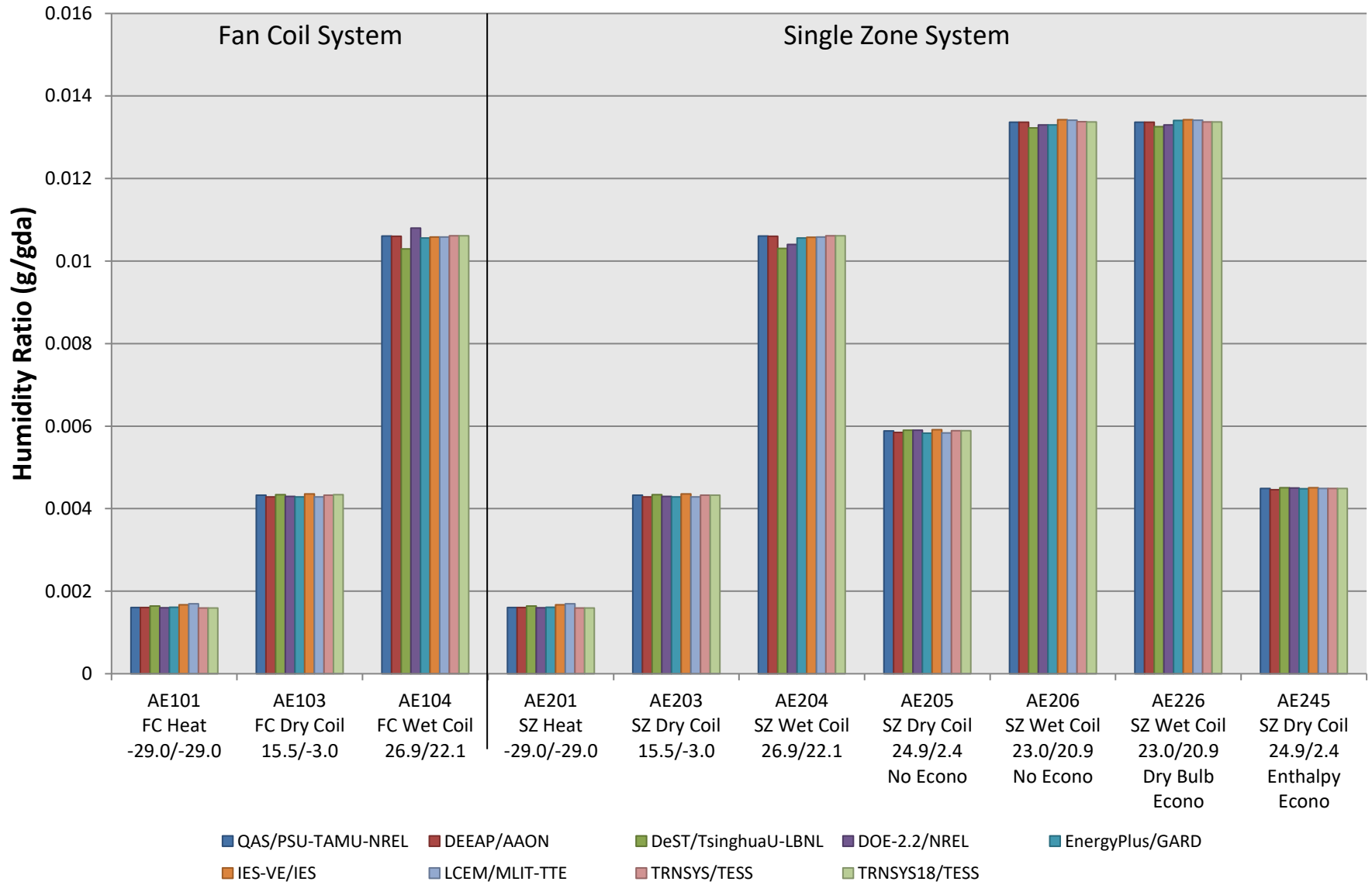
Figure B16.7.1-12. FC/SZ Supply Air Humidity Ratio
