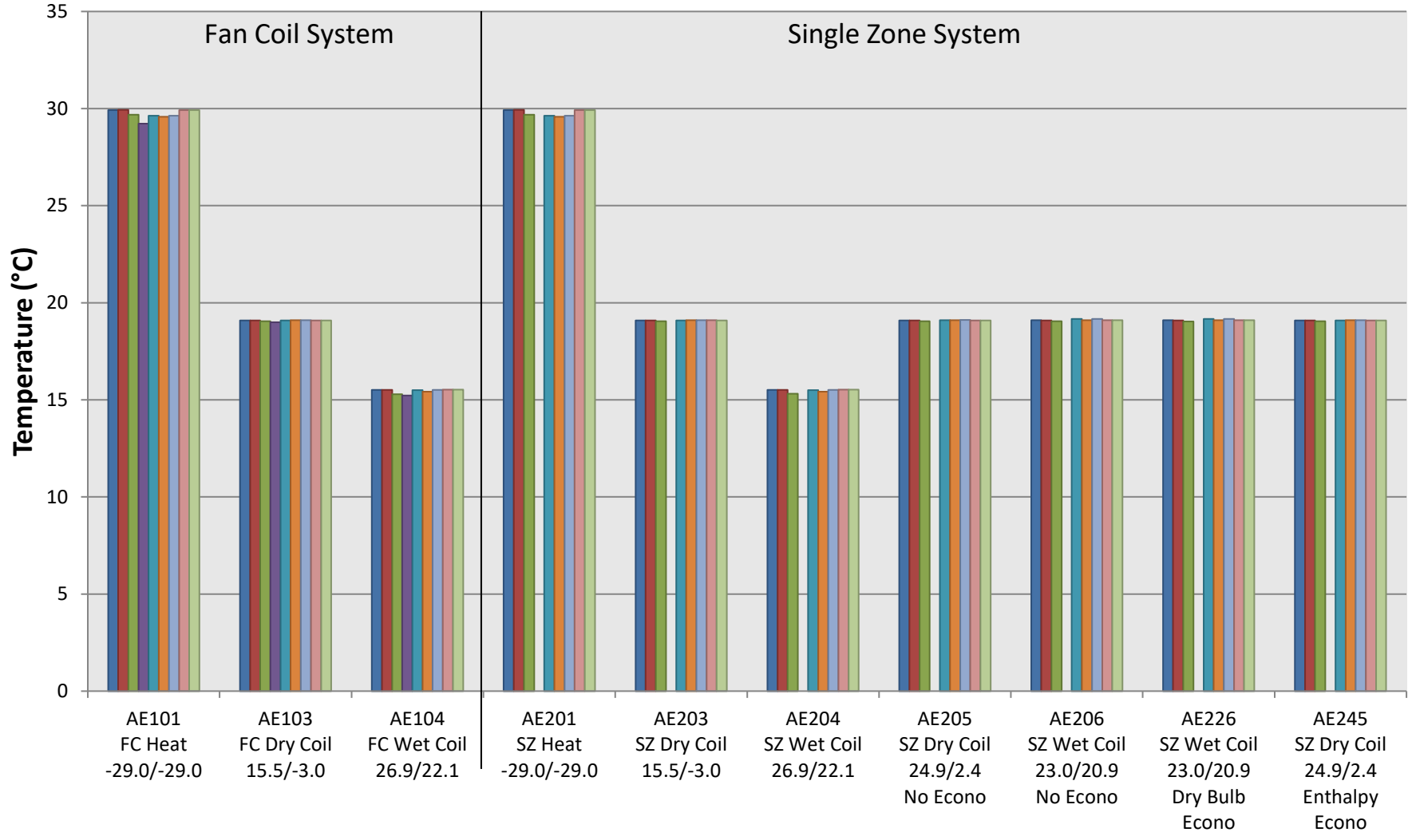
Figure B16.7.1-11. FC/SZ Supply Air Temperature
