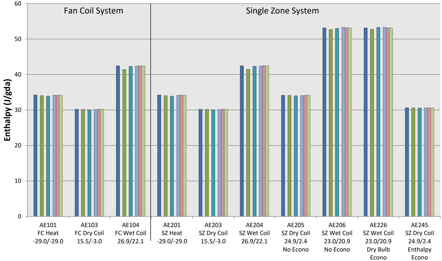
2024 Figure B16.7.1-14. FC/SZ Supply Air Enthalpy
