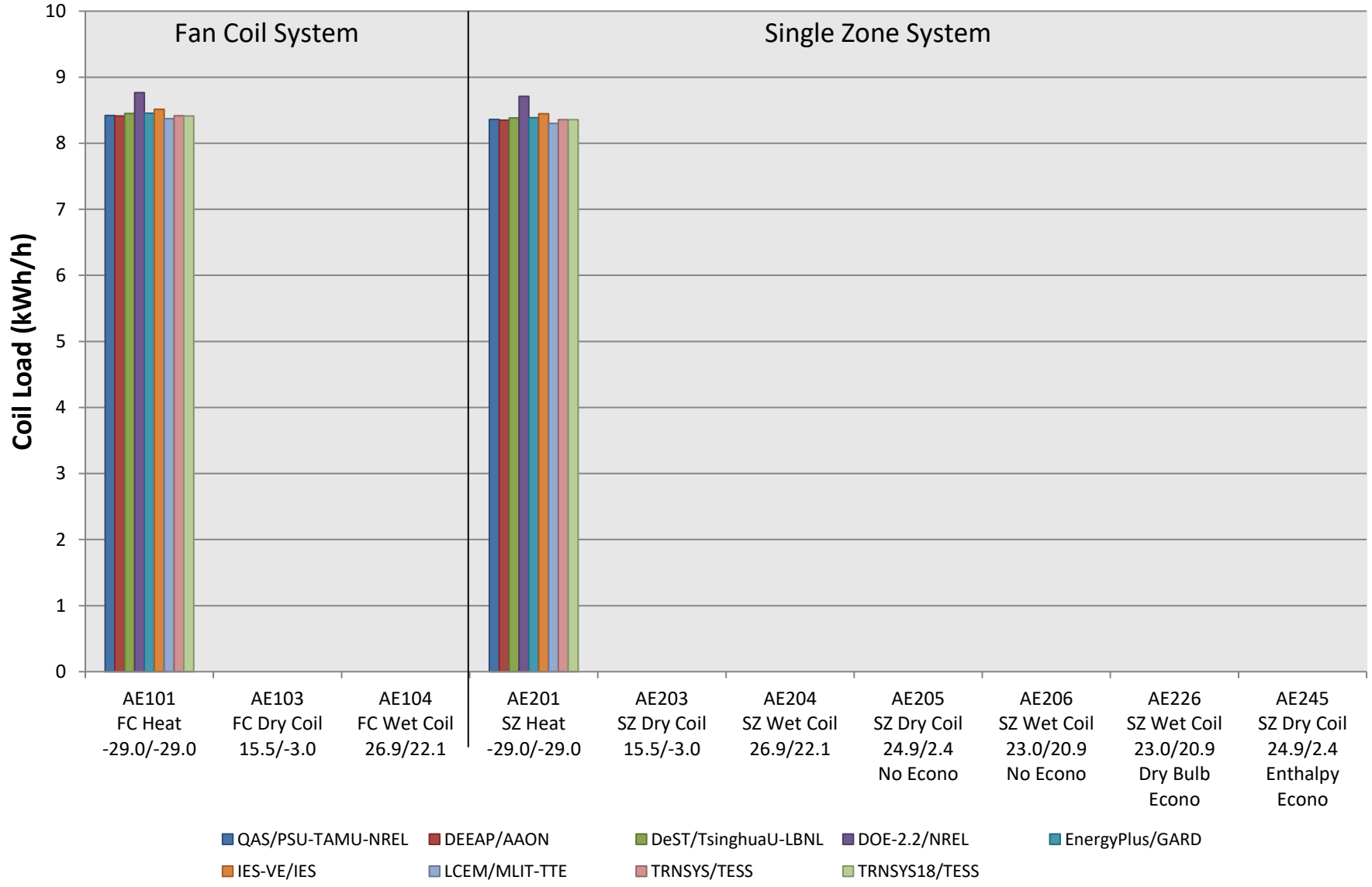
2024 Figure B16.7.1-1. FC/SZ Heating Coil Load [QH]
