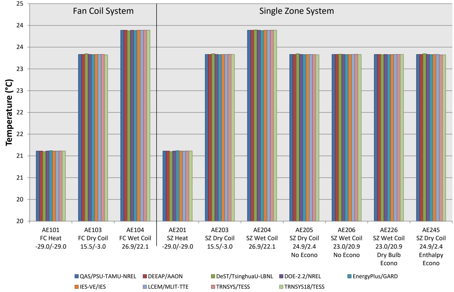
Figure B16.7.1-17. FC/SZ Zone Air Temperature
