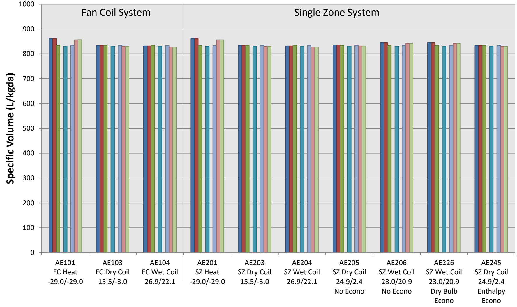
Figure B16.7.1-13. FC/SZ Supply Air Specific Volume
