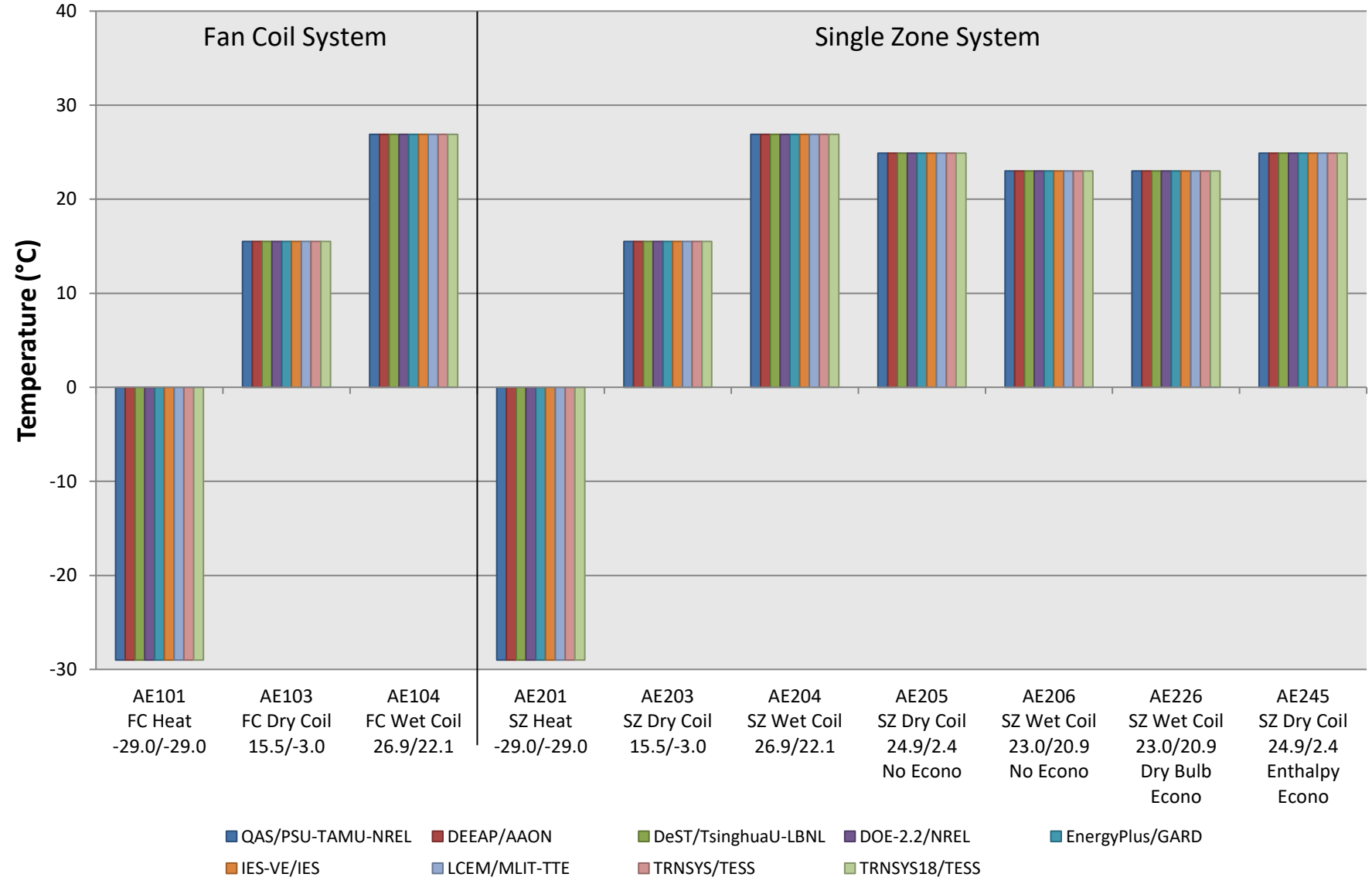
2024 Figure B16.7.1-5. FC/SZ Outdoor Air Temperature
