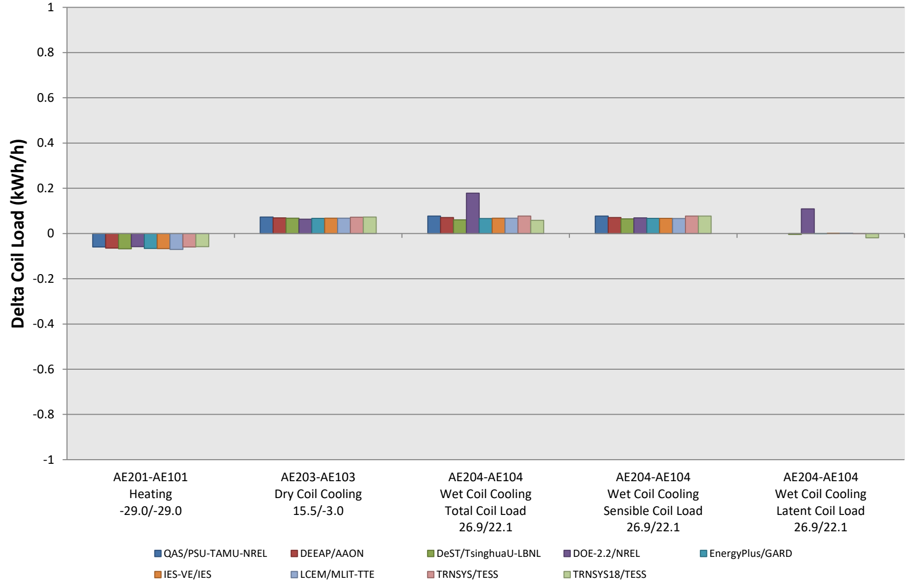
2024 Figure B16.7.1-21. FC/SZ Delta Coil Load, SZ - FC
